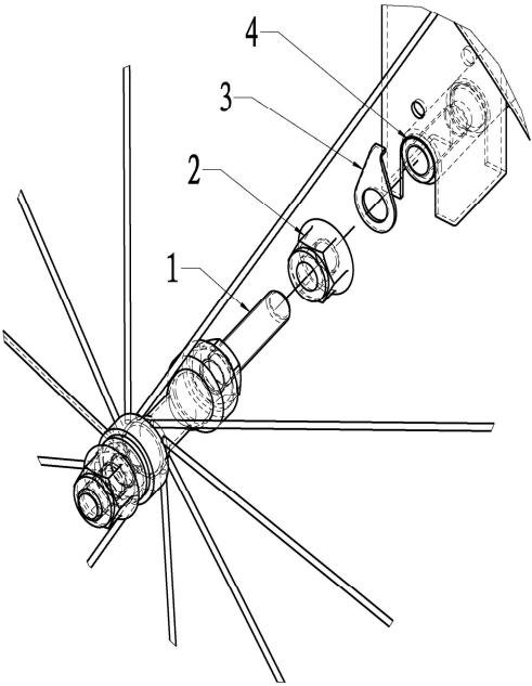
Detail A Proportion 1:1
